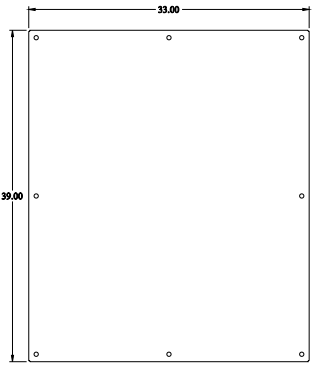
INNER PANEL
