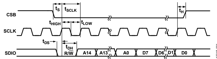
Figure 148. SPI Write Operation Timing
