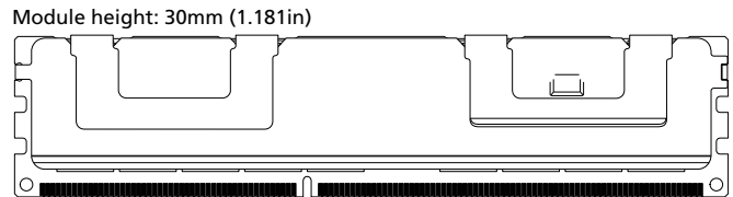
Figure 1: 240-Pin RDIMM (R/C AB)
