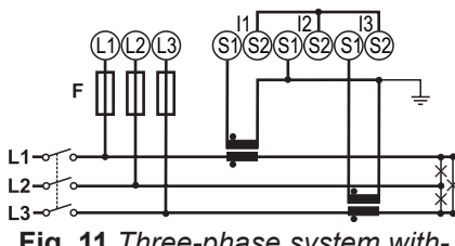
Fig. 11 Three-phase system without neutral (3-wire) unbalanced load and 2 CT (Aron). 315 mA fuse (F).
