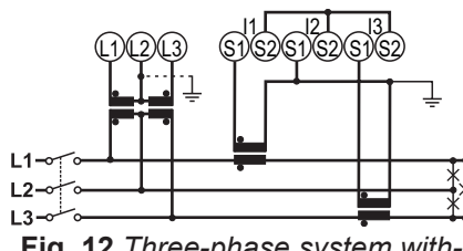
Fig. 12 Three-phase system without neutral (3-wire), unbalanced load, 2 CT (Aron) and 2 VT/PT.
