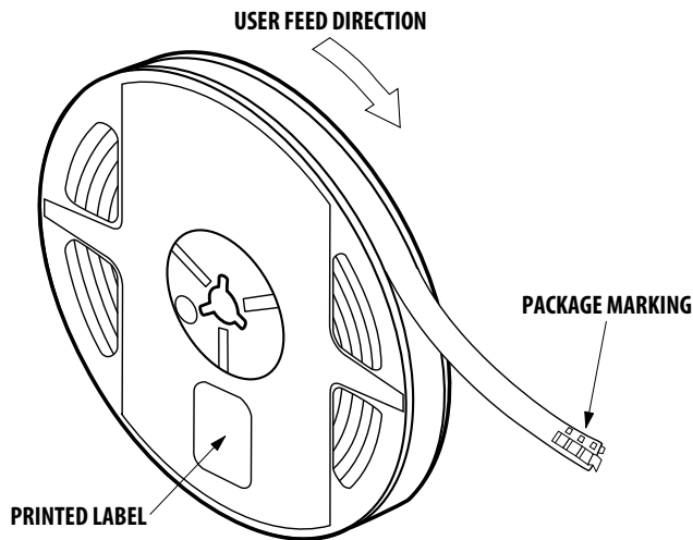
Figure 16 Reeling Orientation
