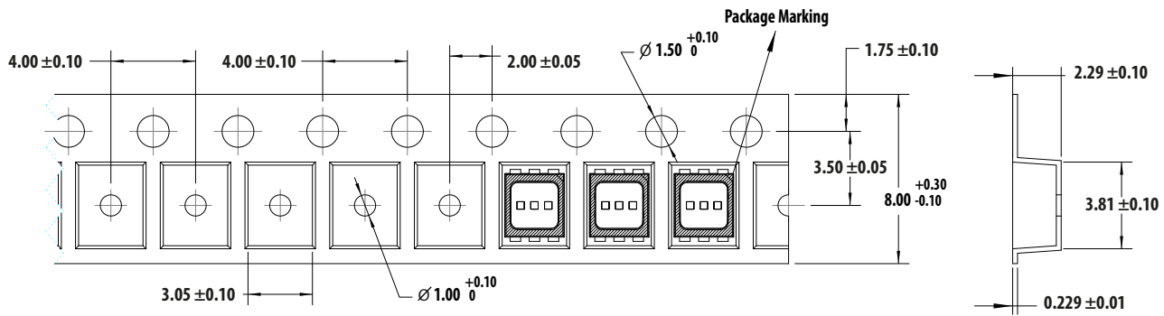
Figure 16 Reeling Orientation
