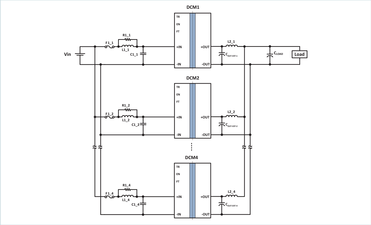
Typical Application 1: DCM4623xD2H26F0yzz in an array of four units
