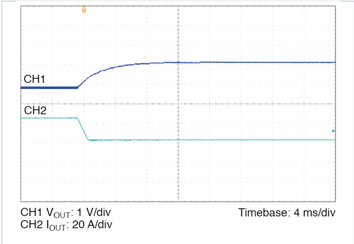
Figure 7 — 100% to 10% load transient response, V_{IN} = 300\text{ V} , nominal trim, C_{OUT\_EXT} = 1000\ \mu\text{F}
