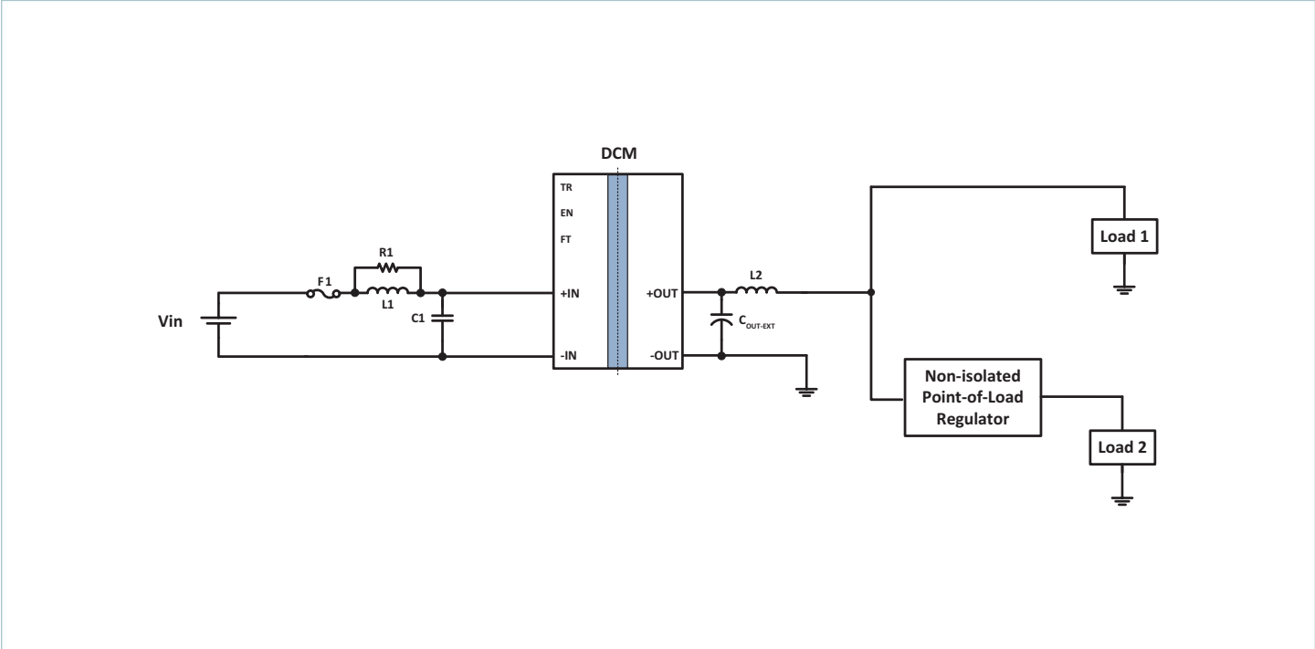
Typical Application 2: Single DCM4623xD2H26F0yzz, to a non-isolated regulator, and direct to load
