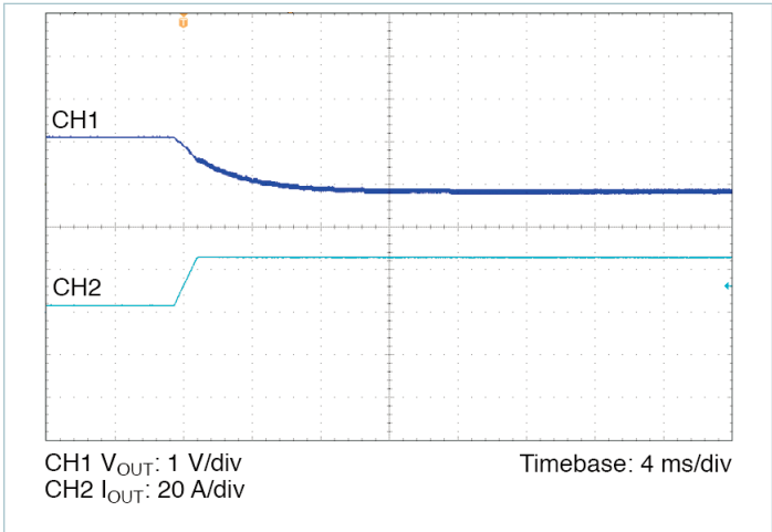
Figure 8 — 10% to 100% load transient response, V_{IN} = 300\text{ V} , nominal trim, C_{OUT\_EXT} = 1000\ \mu\text{F}
