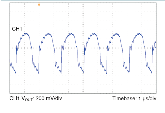
Figure 19 — Output voltage ripple, V_{IN} = 300\text{ V} , V_{OUT} = 24.0\text{ V} , C_{OUT\_EXT} = 1000\text{ }\mu\text{F} , R_{LOAD} = 0.960\text{ }\Omega
