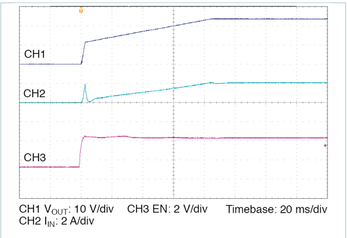
Figure 17 — Startup from EN, V_{IN} = 300\text{ V} , C_{OUT\_EXT} = 10000\text{ }\mu\text{F} , R_{LOAD} = 0.960\text{ }\Omega
