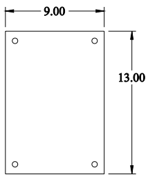
INNER PANEL
