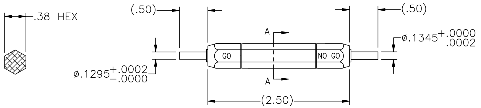
SECTION A - A
