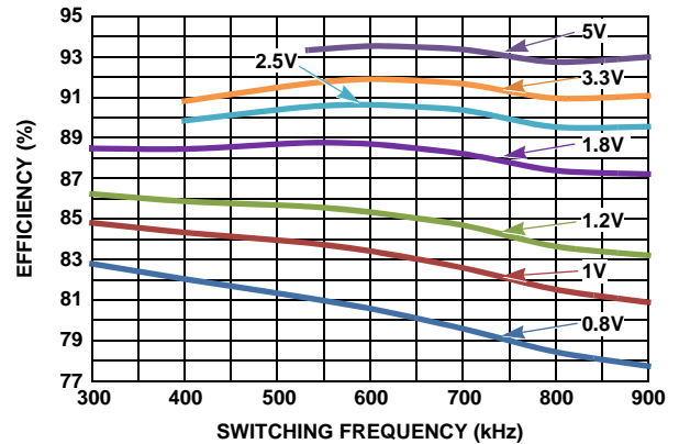
FIGURE 4. EFFICIENCY vs SWITCHING FREQUENCY AT V_{IN} = 12V AND I_{OUT} = 33A FOR VARIOUS OUTPUT VOLTAGES
