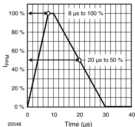
20548 Fig. 2 - 8/20 \mu s Peak Pulse Current Wave Form acc. IEC 61000-4-5
