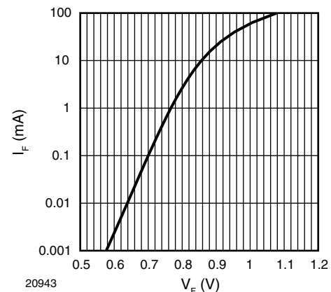
20943 Fig. 4 - Typical Forward Current I_F vs. Forward Voltage V_F
