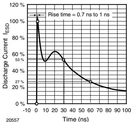
20557 Fig. 1 - ESD Discharge Current Wave Form acc. IEC 61000-4-2 (330 \Omega /150 pF)
