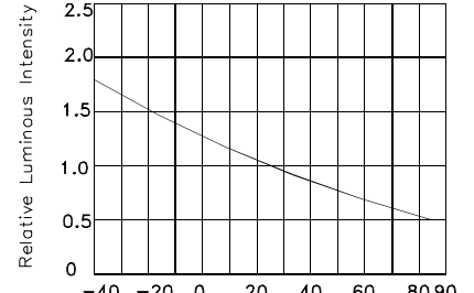
Ambient Temperature TA (°C) LUMINOUS INTENSITY Vs. AMBIENT TEMPERATURE
