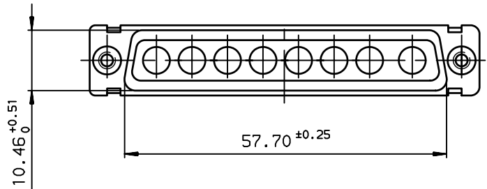
LAYOUT DIMENSIONS (after plating) CONNECTOR SIDE VIEW
