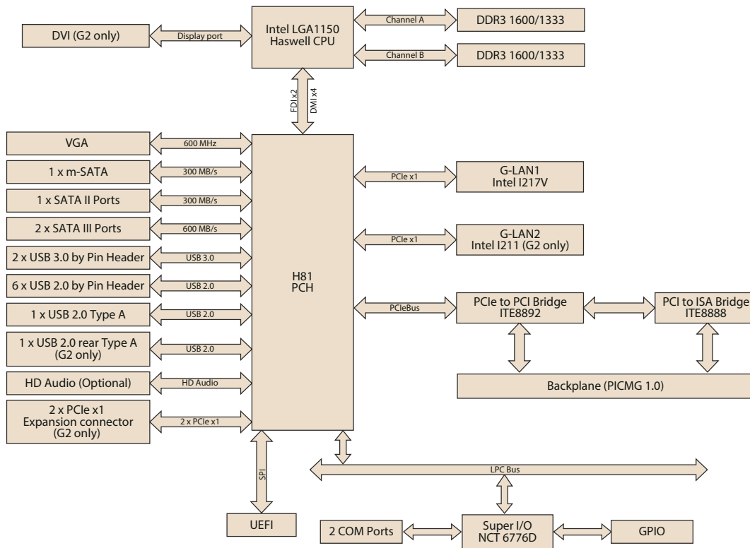
Figure 1.2 PCA-6028 Block Diagram
