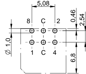
RECOMMENDED LAYOUT
