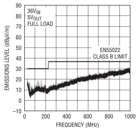
Radiated Emissions
