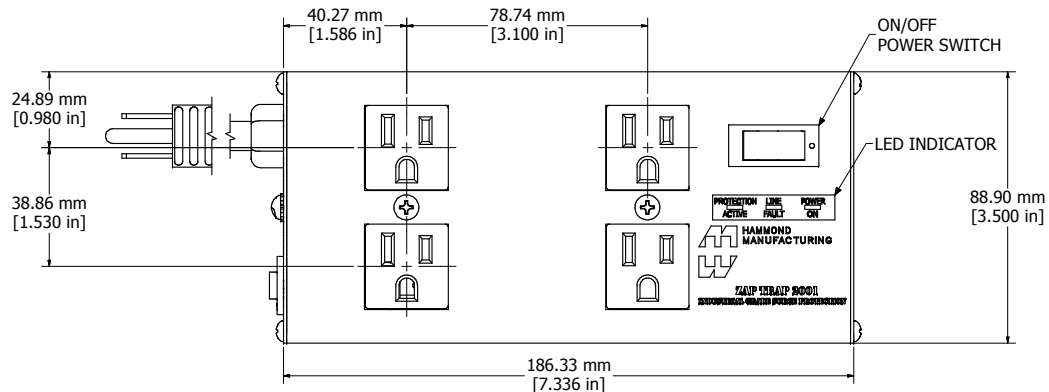
ASSEMBLY - VIEW FROM TOP
