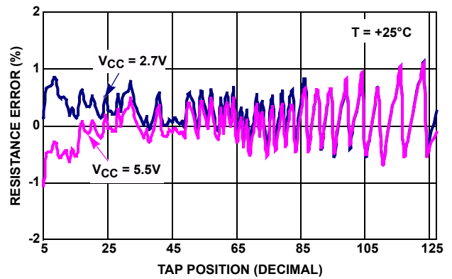
FIGURE 2. RESISTANCE ERROR vs TAP POSITION [(RW) = V CC /R TOTAL ] FOR 10kΩ (W)
