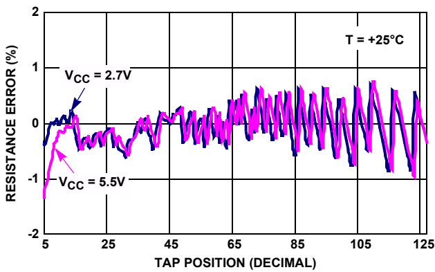
FIGURE 1. RESISTANCE ERROR vs TAP POSITION [(RW) = V CC /R TOTAL ] FOR 100kΩ (T)
