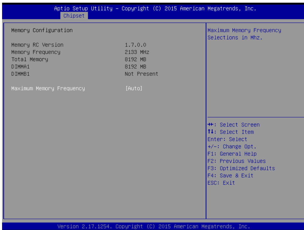
Figure 3.25 Memory Information
