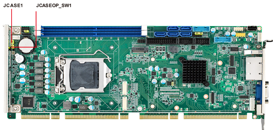
Figure 2.1 Case Open Jumper Locations
