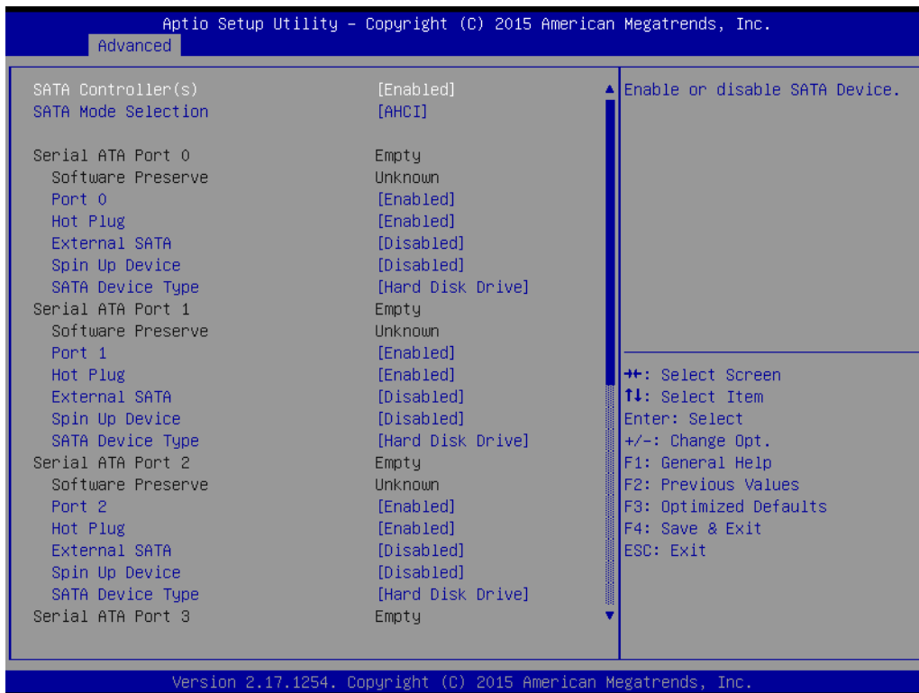
Figure 3.17 SATA Configuration
