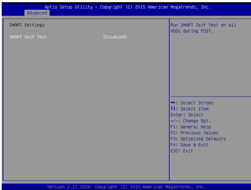
Figure 3.8 Smart Setting
