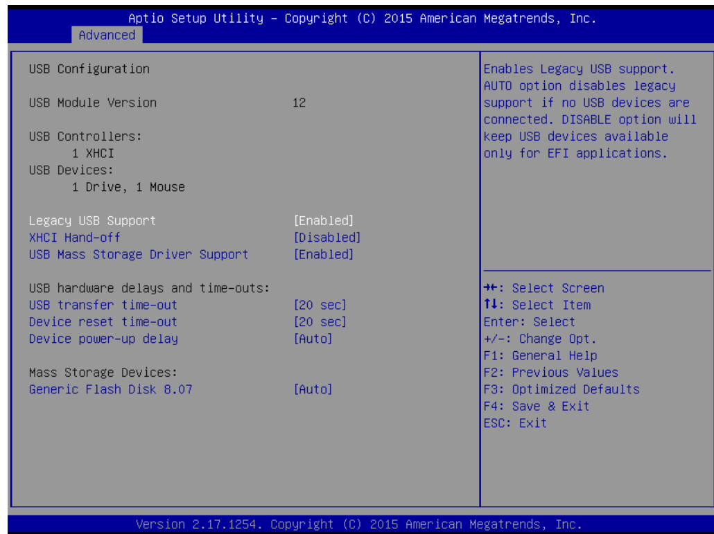
Figure 3.20 USB Configuration
