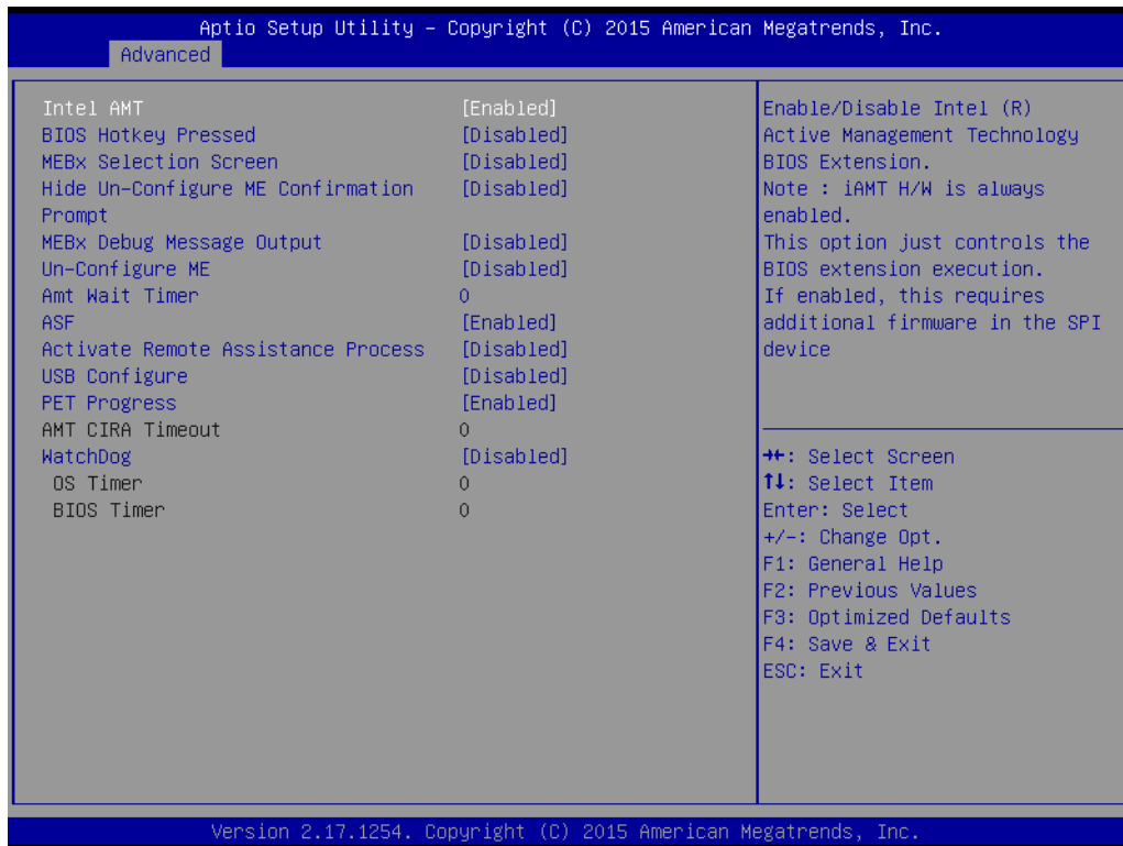
Figure 3.6 AMT Configuration
