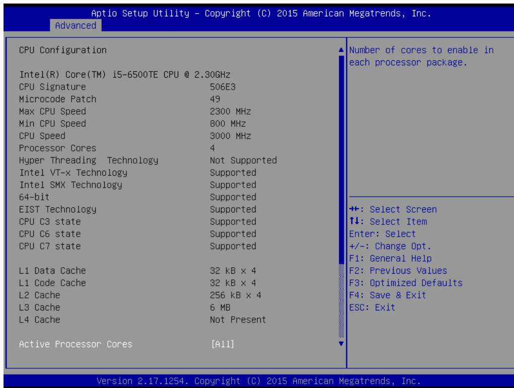
Figure 3.15 CPU Configuration
