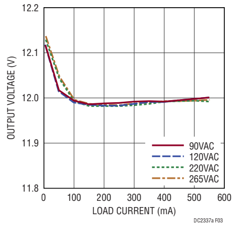
Figure 3. Load and Line Regulation
