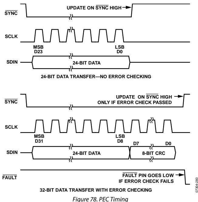
Figure 78. PEC Timing
