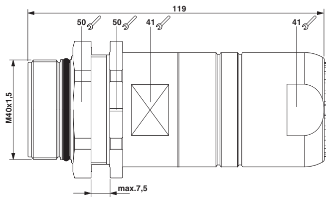
Dimensioned drawing
