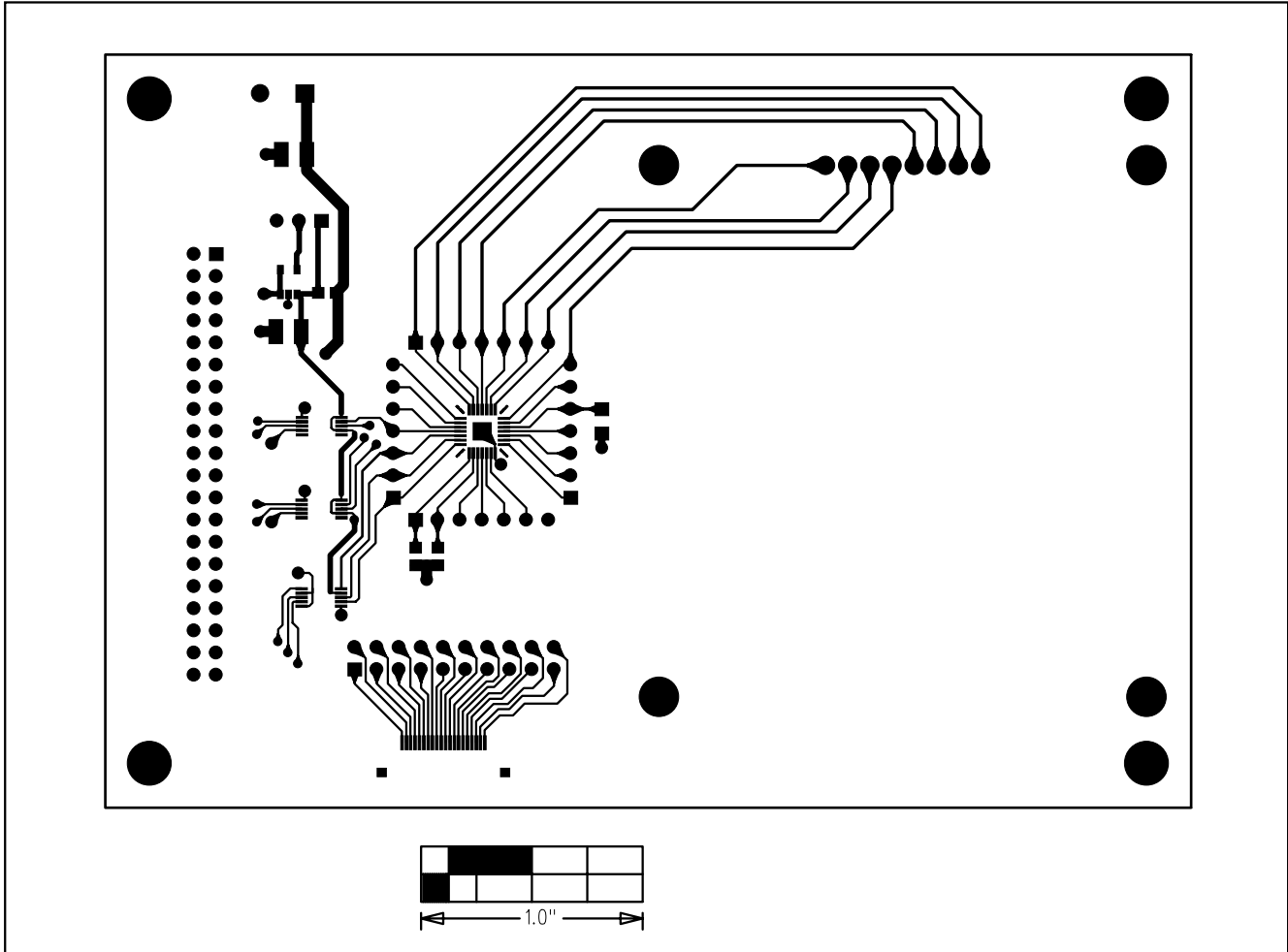
Figure 11. MAX1234 EV Kit PC Board Layout—Component Side
