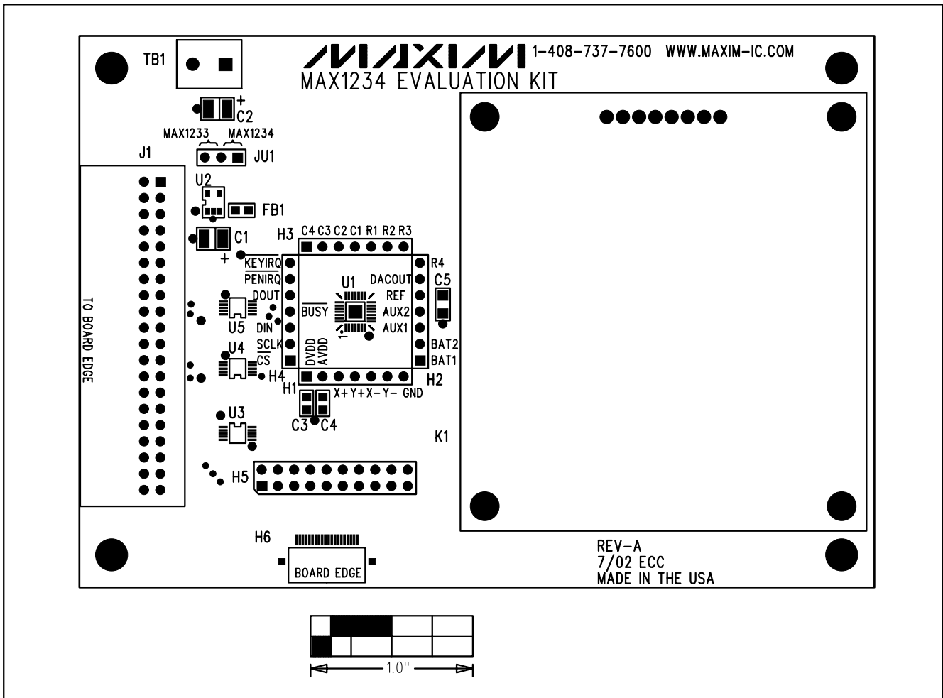
Figure 10. MAX1234 EV Kit Component Placement Guide—Component Side
