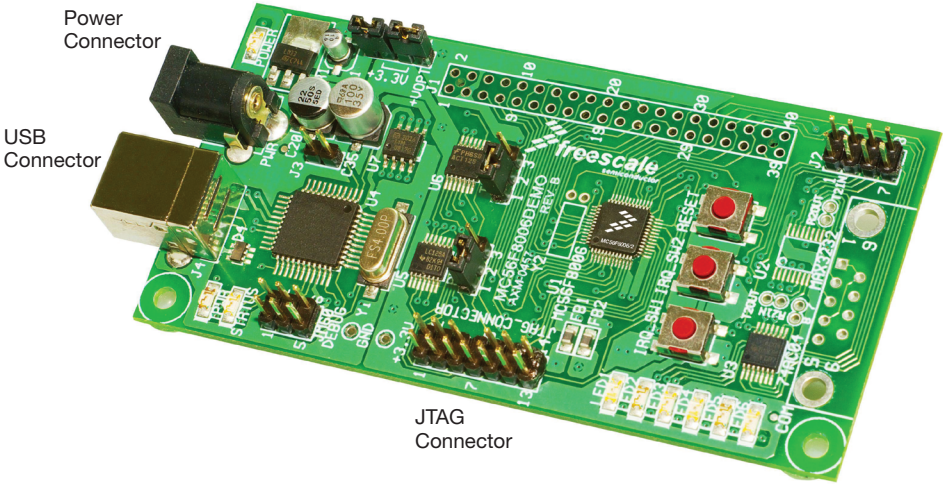
Figure 1. MC56F8006DEMO
