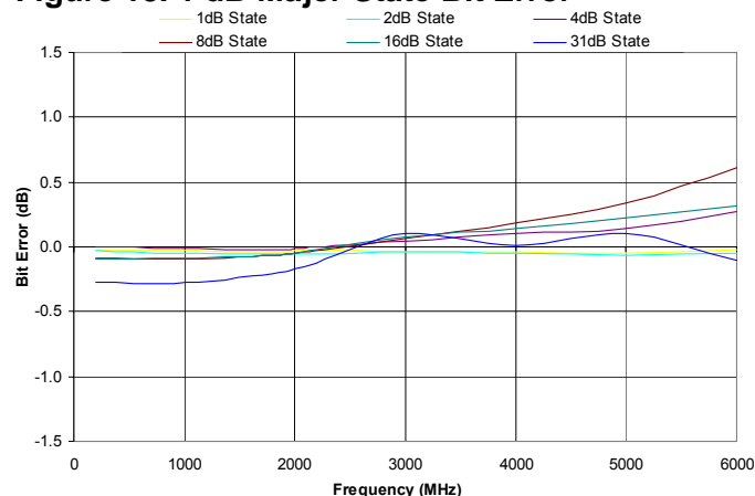
Figure 13. 1 dB Major State Bit Error
