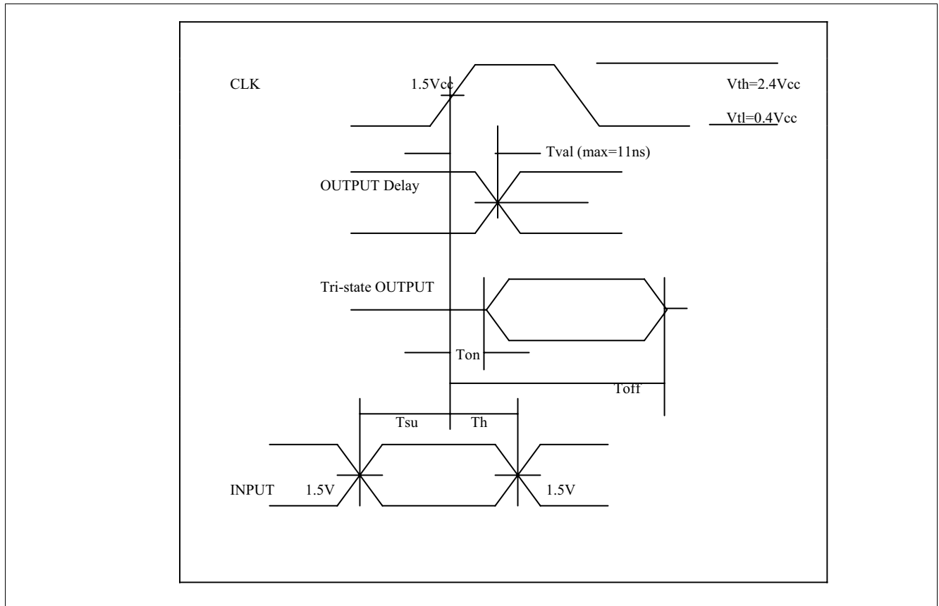
Figure 18 PCI Timings
