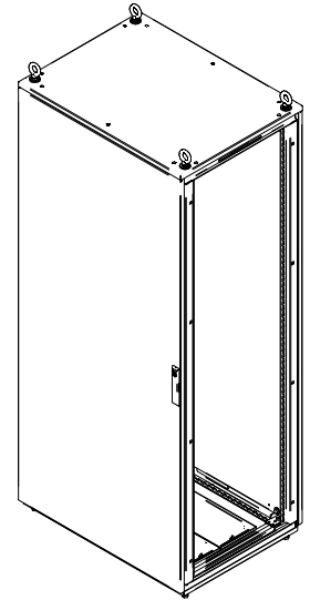
ISOMETRIC
