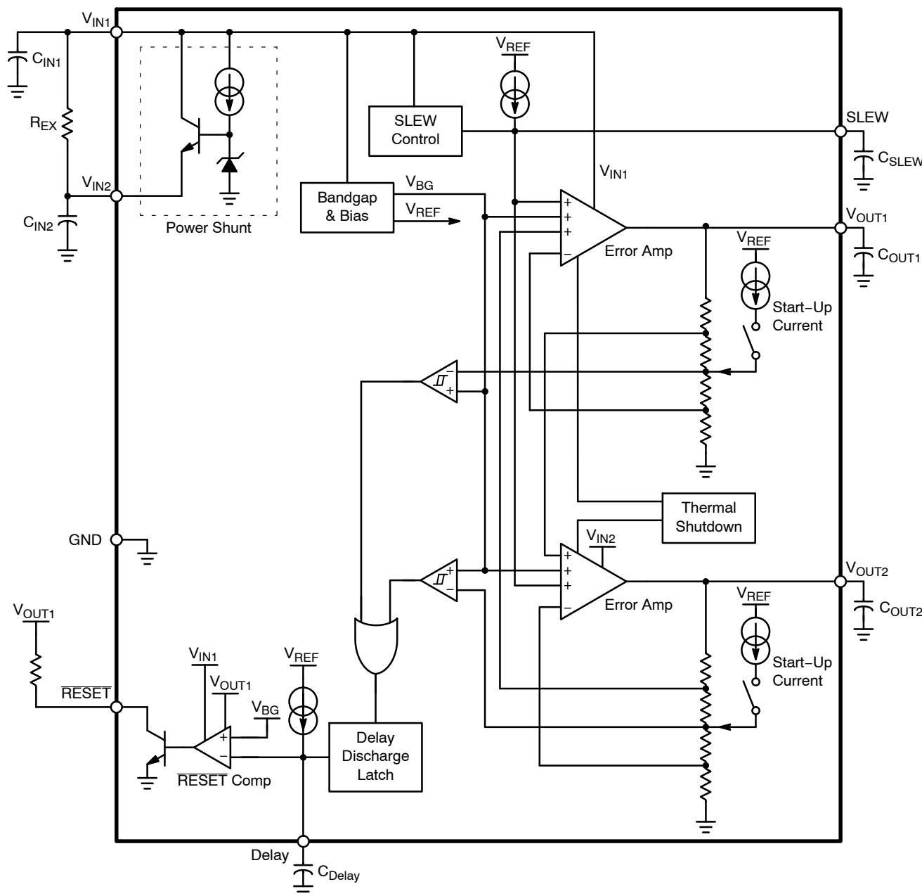
Figure 2. Block Diagram
