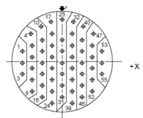
Contact Layout
