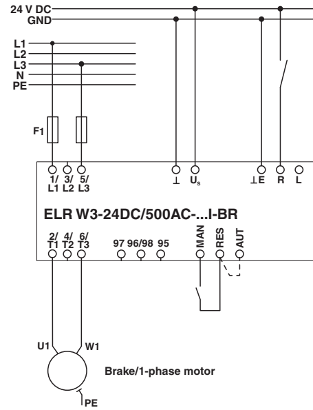
Circuit diagram
