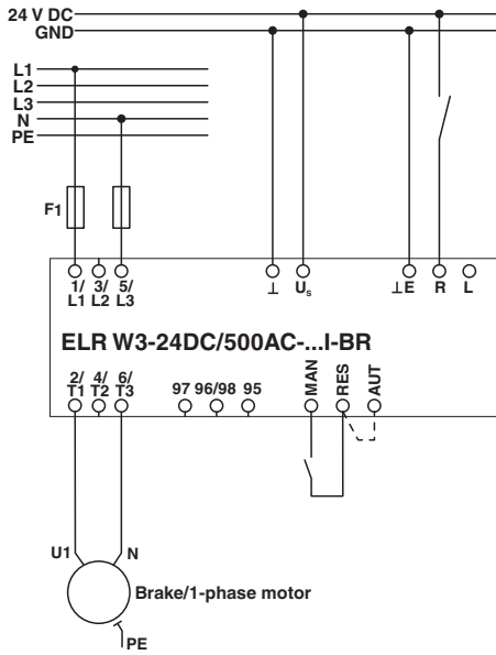
Circuit diagram
