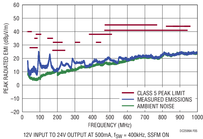
Figure 5. CISPR25 Radiated Emissions Test, Peak Detection
