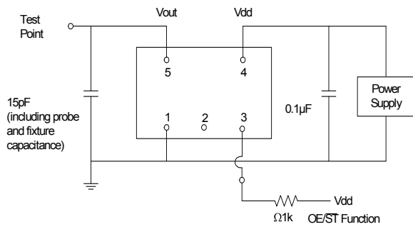
Figure 2. Test Circuit
