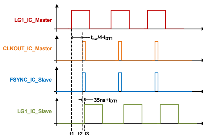
FIGURE 65. TIMING DIAGRAM OF CLKOUT vs LG1 AND FSYNC vs LG1 (CLKOUT_MASTER CONNECTED TO FSYNC_SLAVE)
