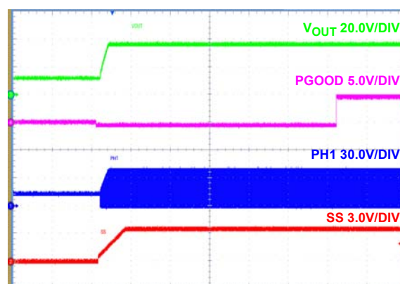
FIGURE 8. SOFT-START, CCM MODE (DE/PHDRP = GND), I_{OUT} = 8A
