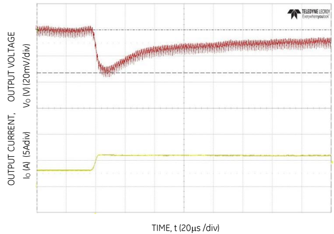
Figure 16. Transient Response to Dynamic Load Change from 50% to 100% at 12V in , C out =3x47µF+1x330µF, CT tune =3900pF, RT tune =300
