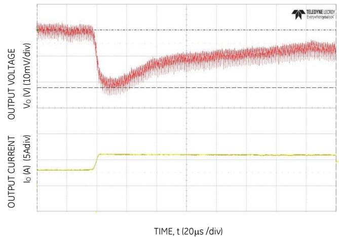
Figure 10. Transient Response to Dynamic Load Change from 50% to 100% at 12Vin, Cout=3x47uF+2x330uF, CTune=5600pF, RTune=300Ω
