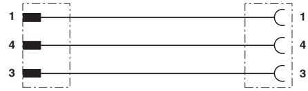
Contact assignment of M12 connector/socket
