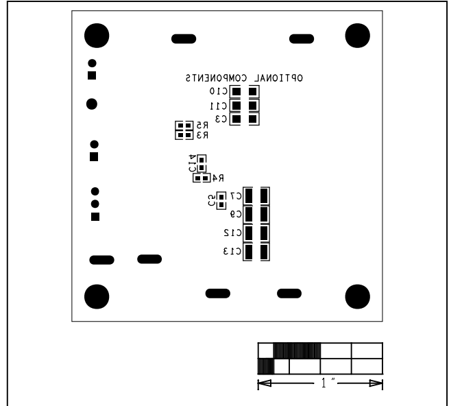
Figure 2. MAXM17545 EV Kit Component Placement Guide—Solder-Side
