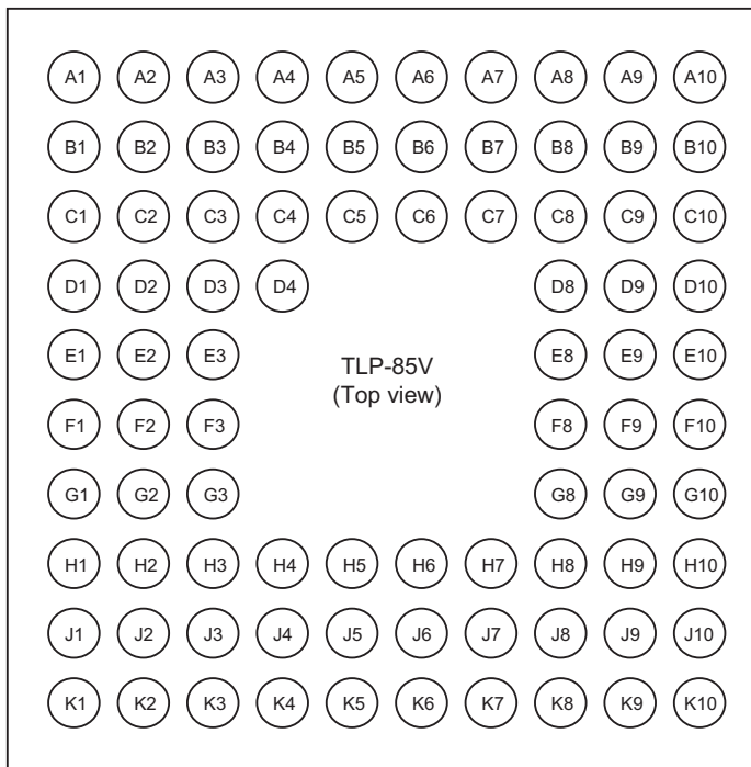
Figure 1.4 Pin Arrangement (TLP-85V, H8/38024R Group, H8/38024S Group)
