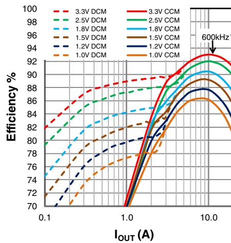
Figure 21: Efficiency, V_{IN}=12\text{V}
