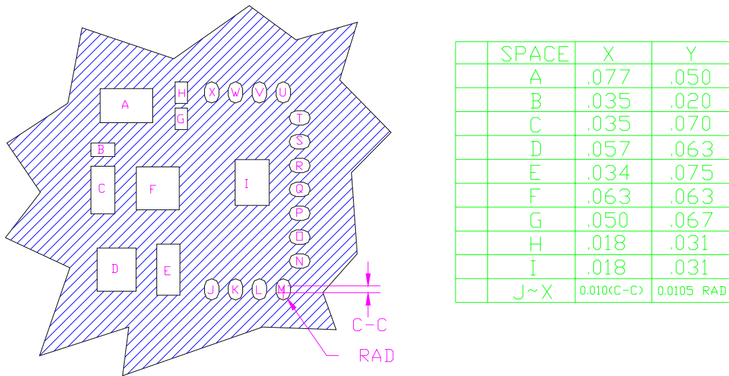
SQUEEGEE VIEW RECOMMENDED STENCIL OPENING ALL DIMENSIONS IN INCHES
