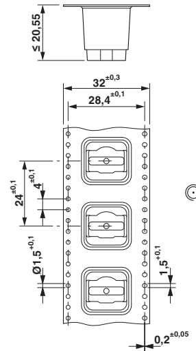
Dimensional drawing
