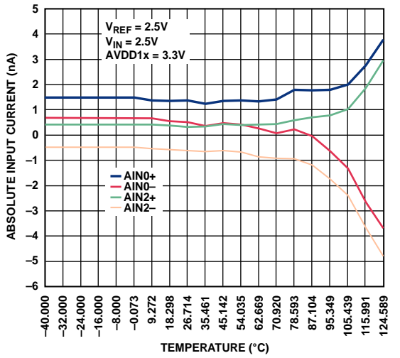
Figure 57. Absolute Input Current vs. Temperature, High Resolution Mode
