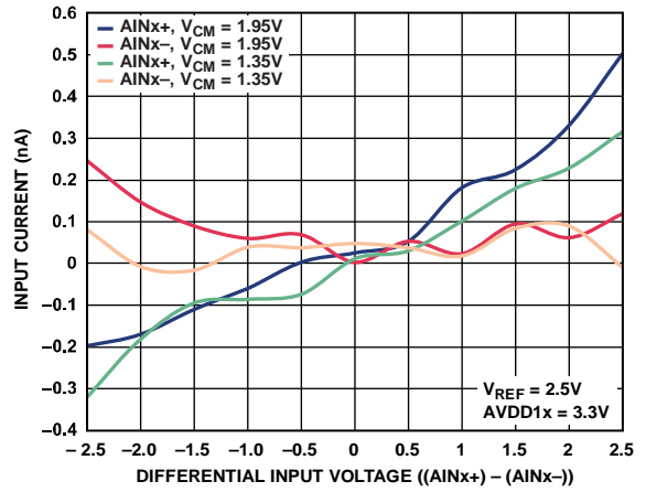
Figure 59. Input Current vs. Differential Input Voltage, Low Power Mode
