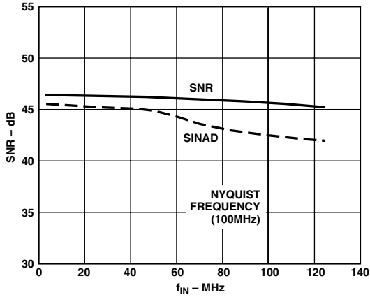
TPC 1. SNR vs. f_{IN} : f_S = 200 MSPS
