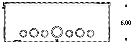
BOTTOM VIEW
