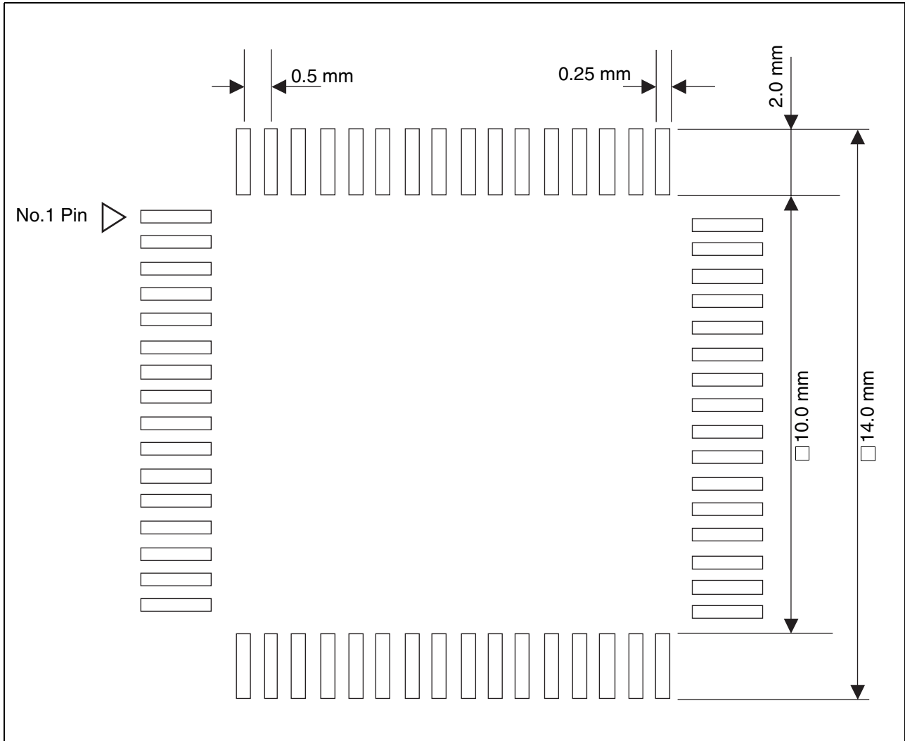
Figure 3 Recommended Footprint Dimensions for Mounting the NQPACK
