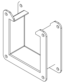
ISOMETRIC VIEW
