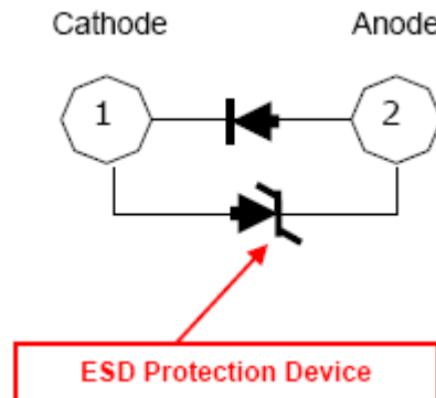
Circuit
