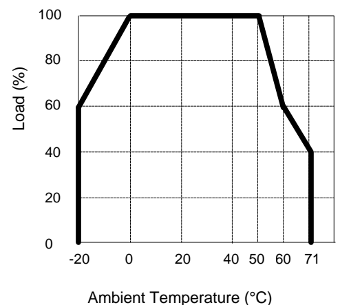
OUTPUT DERATING
