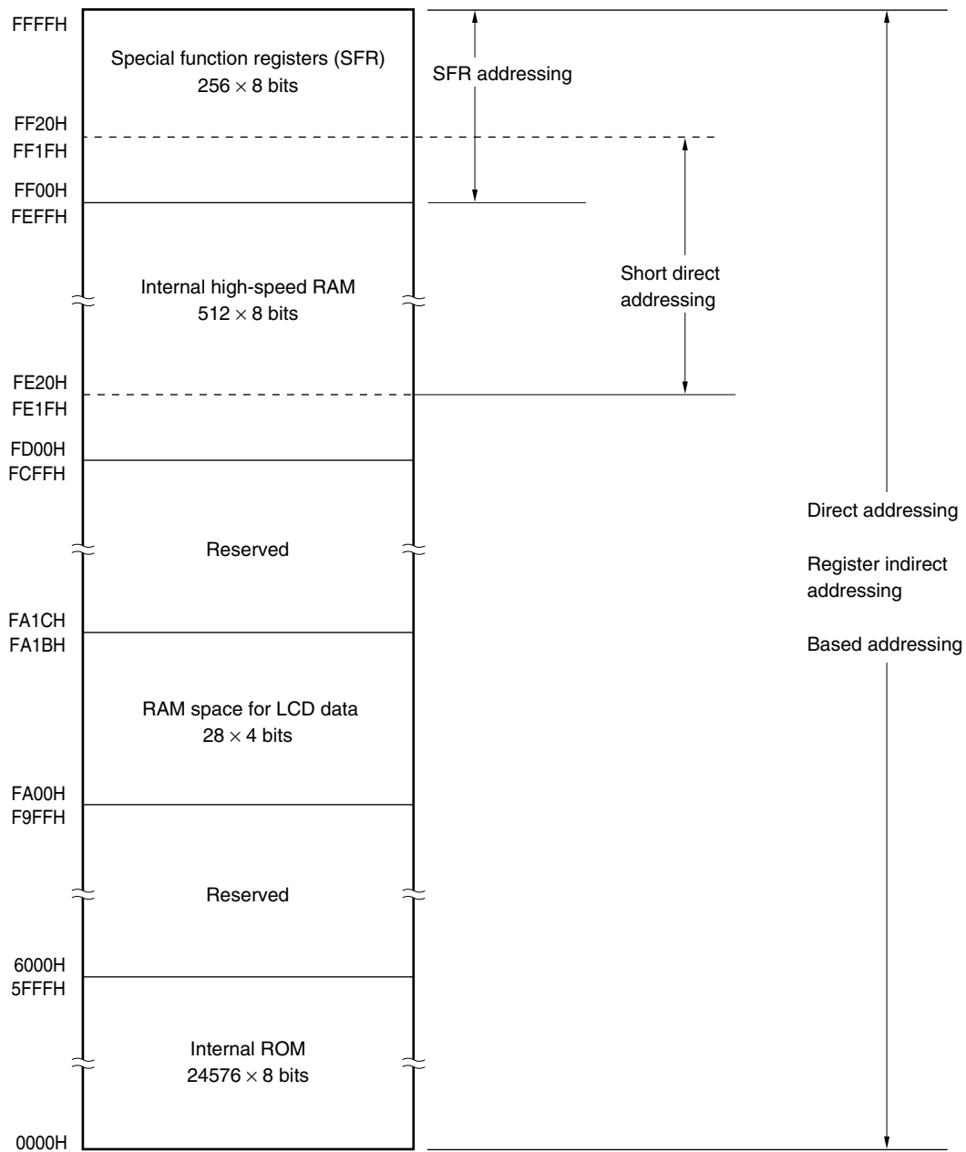
Figure 3-7. Data Memory Addressing ( \mu PD789407A and \mu PD789417A)
