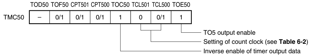
Figure 6-6. Settings of 16-Bit Timer Mode Control Register 50 for Timer Output Operation
