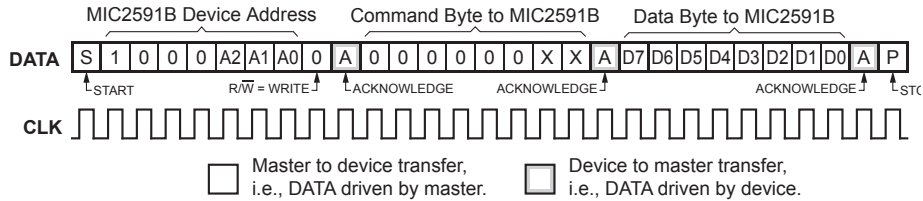
Figure 10. WRITE_BYTE Protocol
