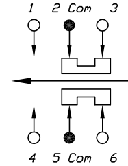
CIRCUIT: DPDT CONTACT CONFIGURATION
